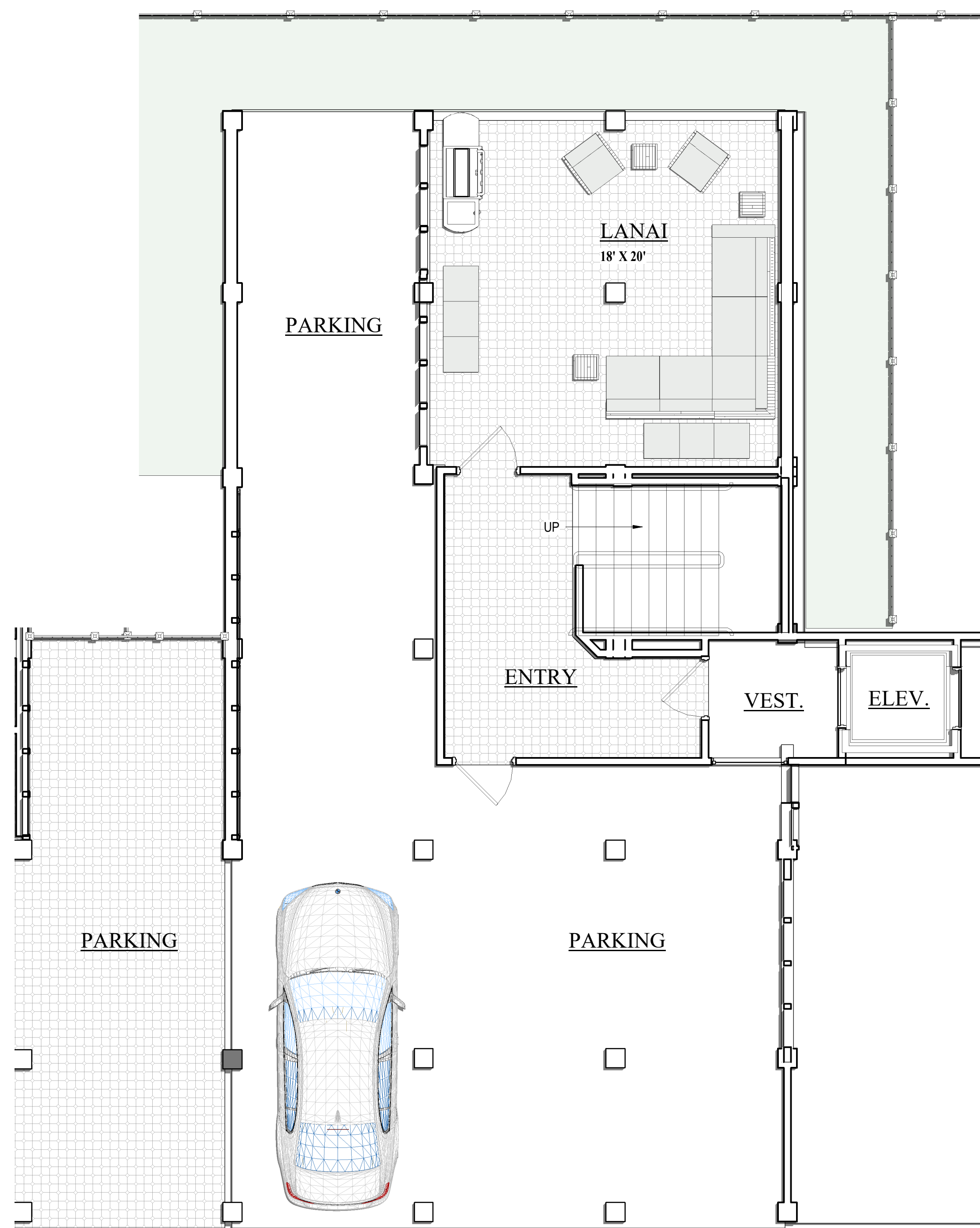
UNIT 7 LEVEL 1 FLOOR PLAN
